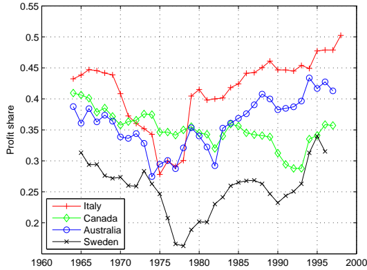
Figure 13: Approximation of \rho .
